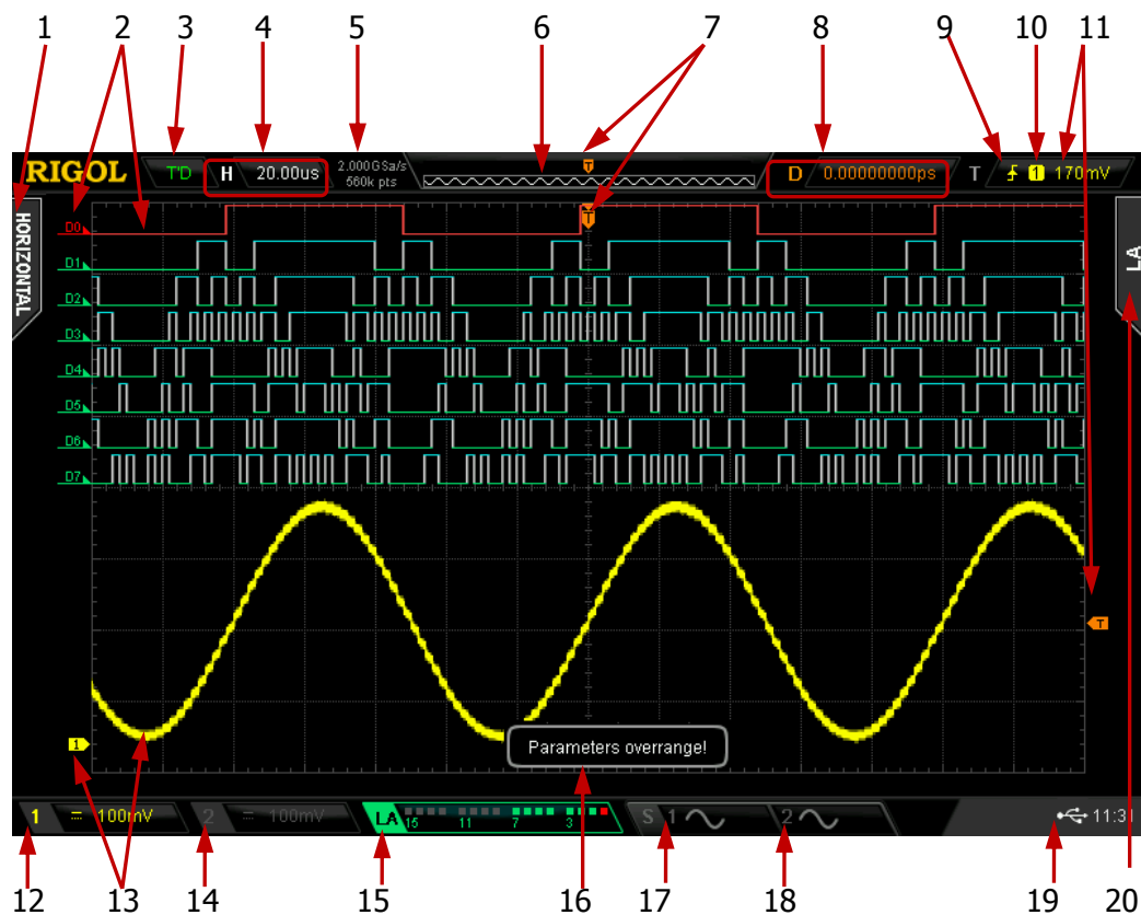
Figure 12 User Interface
